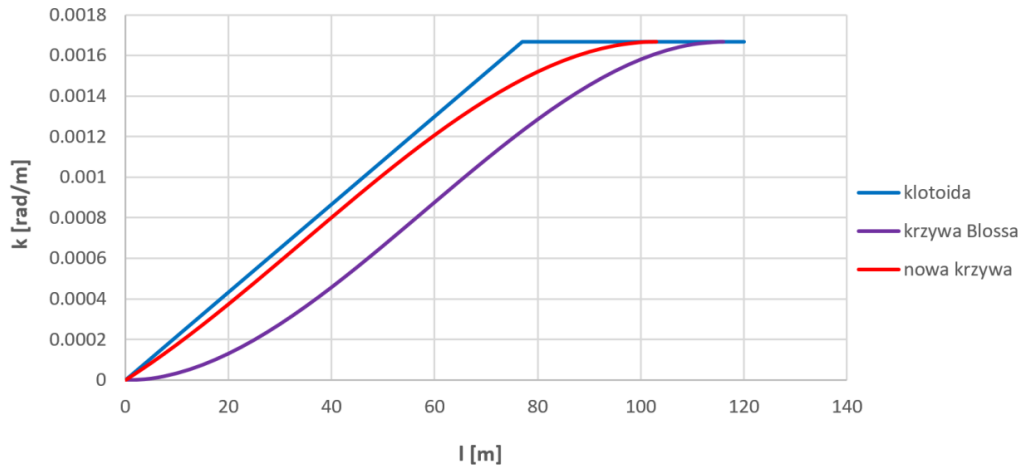
3. Curvature charts along the length of the compared transition curves ( R = 600 \text{ m} )
