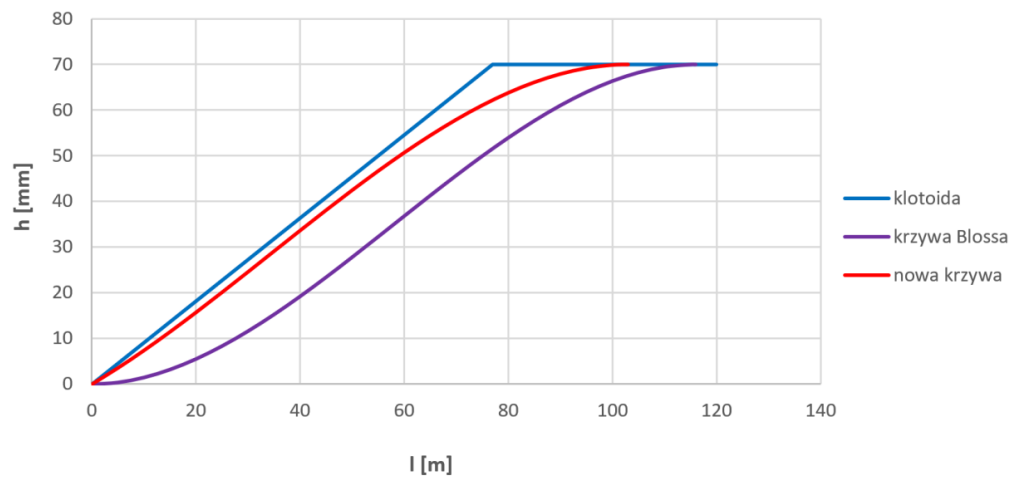
5. Charts of ordinates of the cant ramp over the length of the compared transition curves ( h_0 = 70 \text{ mm} )
